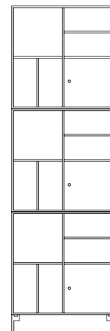
Shelving on legs* W 69.6 cm H 208.8 cm Legs 12.6 cm
