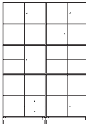
Shelving on legs* W 139.2 cm H 186 cm Legs 12.6 cm
