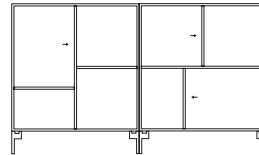
Shelving on legs W 139.2 cm H 69.6 cm Legs H 12.6 cm
